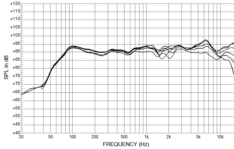
Figure 9— Offaxis Response from 0° to - 50° (anechoic environment)
